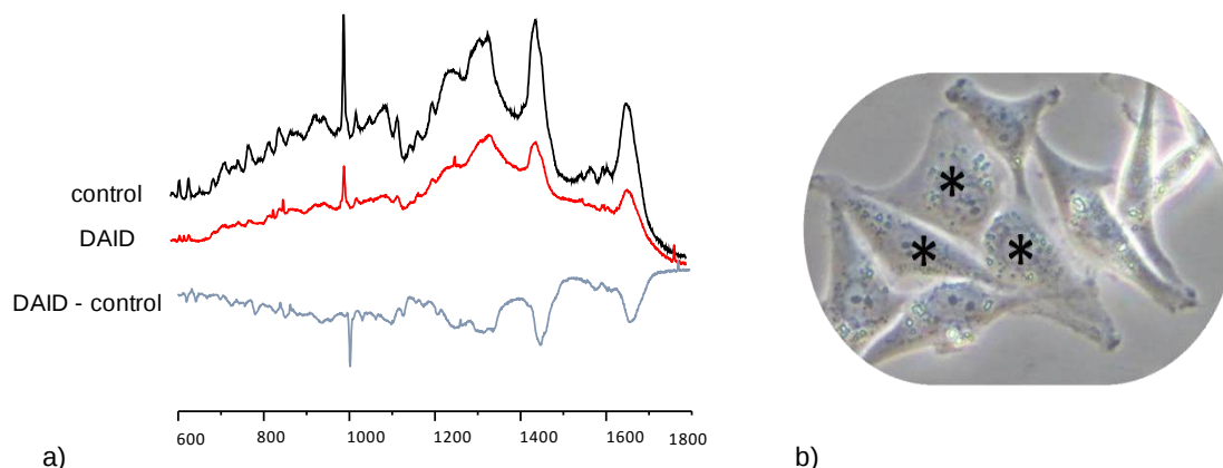
Figure 1: Mean Raman and difference spectra to the control a) and microscopic image of a cell (x100 magnification) showing some points at which data were captured b).
