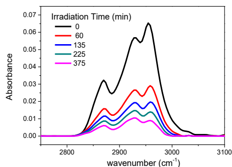
Figure 2: Decay of the CH aliphatic stretching region upon electron irradiation.
