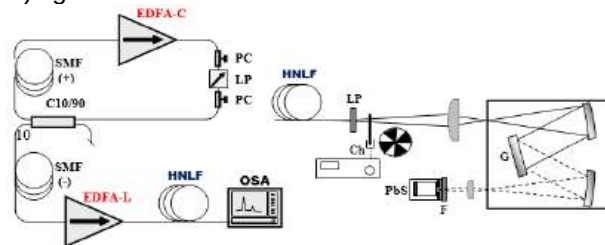
Figure 1. Experimental setup for the supercontinuum generation.
