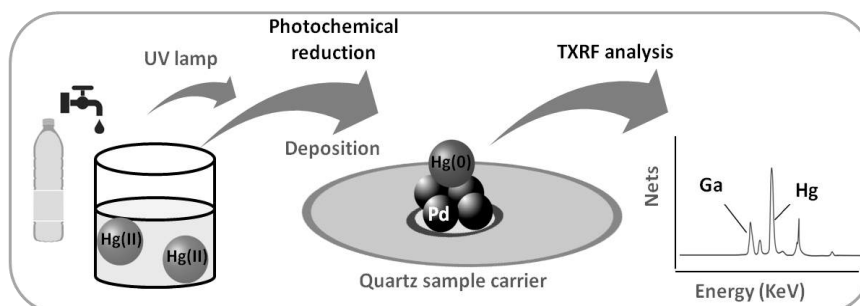
Figure 1. Scheme of the CF-photo CVG approach coupled to TXRF
