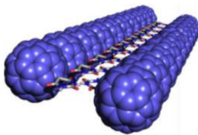
Fig. 2. X-ray structure of a fullerene double-cable.
