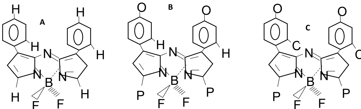
Figure 1. Structure of BODIPYS studied.
