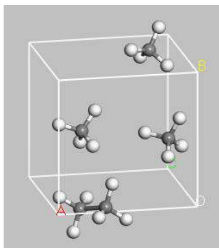
Fig.1. Schematic representation of an amorphous mixture with three methane and one ethane molecules.
