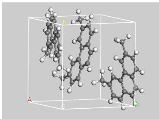
Figure 1: Amorphous cell containing three methylated derivatives of phenanthrene.
