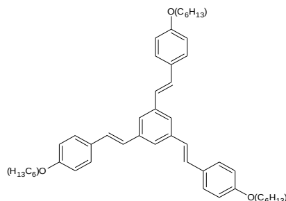
Figure 1. Molecular formula of 1,3,5-tristyrylbenzene
