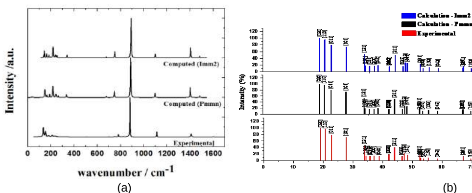
Fig. 1: Calculated and measured rutherfordine Raman spectra and XRD pattern.
