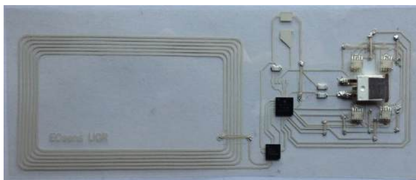
Figure 1. HF RFID tag
