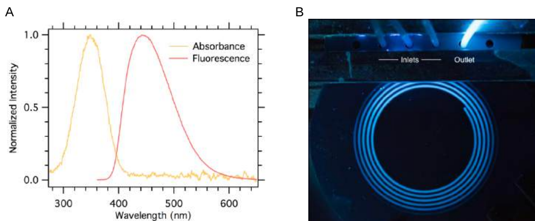
Figure 1. A) Normalized absorption and fluorescence spectra of the Cdots obtained. B) Microfluidic reactor during the synthesis. The increasing fluorescence along the mixer indicates the progress of the reaction.
