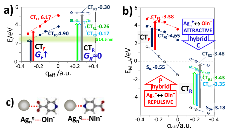
Figure 1. Dependence on q_{\text{eff}} of: (a) TD-M06-HF/LanL2DZ vertical energies (eV) of the forward ( CT_{Fi=0,1} ) and reverse ( CT_{Ri=0-2} ) charge transfer states of silver-isonicotinate complexes [(Ag_n^q-Oin)^{q-1}] , (b) TD-M06-HF/LanL2DZ energies of the same states but referred to the energy of the metallic clusters ( Ag_n^q ) and the adsorbate ( in^- ) at infinite separation ( E_{M...A} ). (c) C_{2v} complexes of isonicotinate bonded to silver through the aromatic nitrogen ( Ag-Nin^- ) or the carboxylate ( Ag-Oin^- ).
