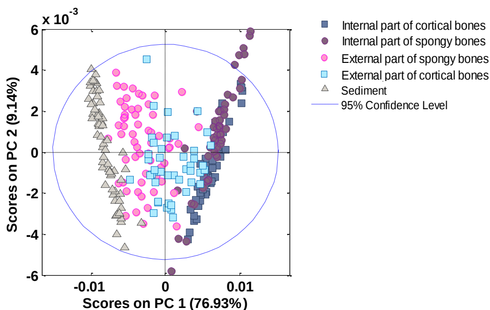
Figure 1. Scores plot for PC1 and PC2 after FD and MC pretreatment for Misericordia and En Gil Necropolises using differentiated internal and external part of bones in spongy and cortical remains.
