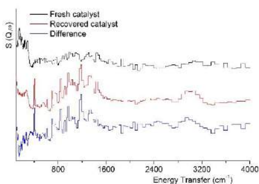
Fig. 2 – INS spectra of Mo heterogeneous catalyst used in styrene oxidation.
