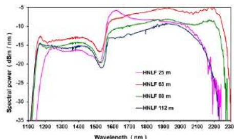
Figure 2. Supercontinuum spectral generated by various lengths of HNLF.
